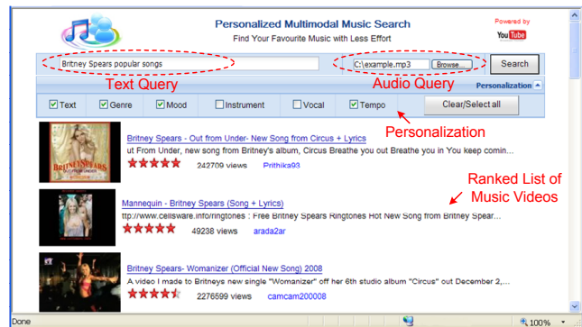
Figure 3: Search interface.
